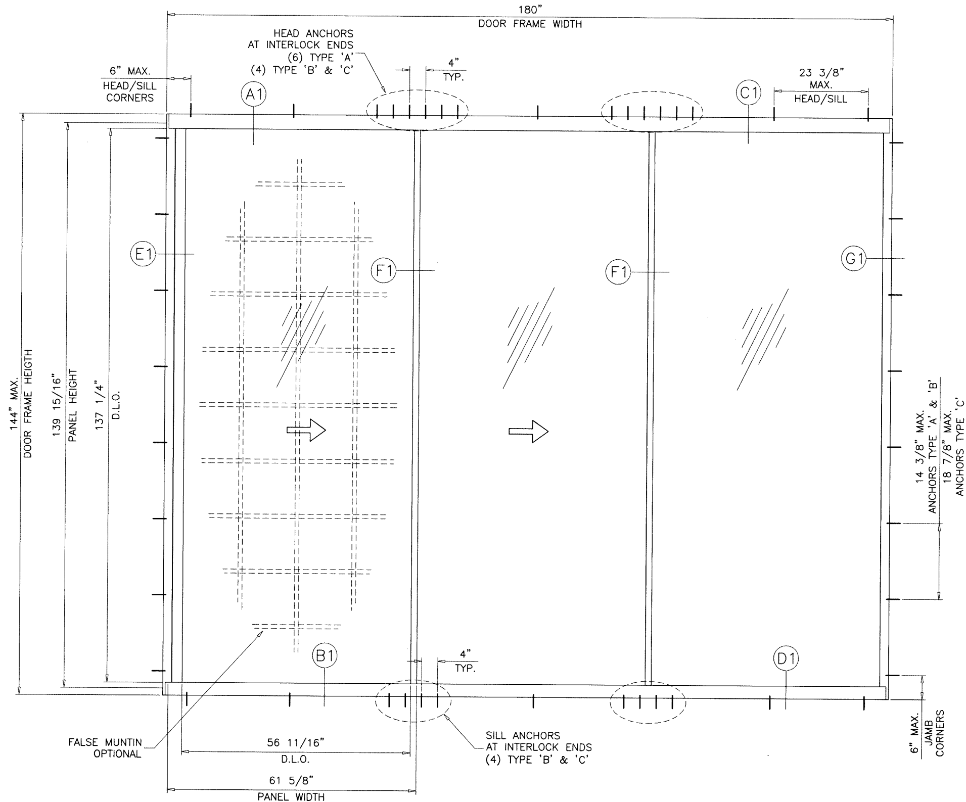
TYPICAL ELEVATION TESTED UNIT (3 TRACK)
