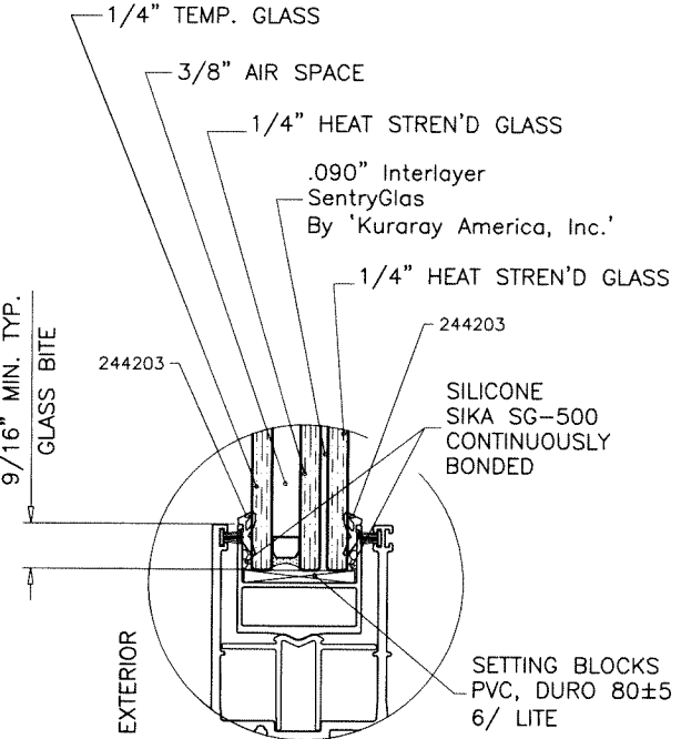
GLASS TYPE 'Ci' 1-3/16" OVERALL INSUL. LAM. GLASS
