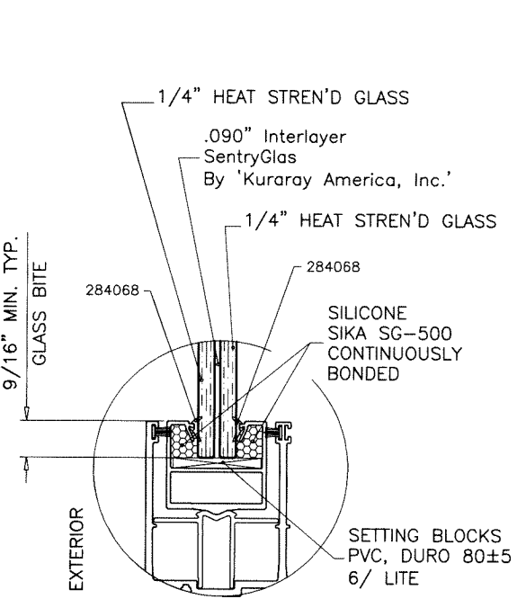
GLASS TYPE 'C' 9/16" OVERALL LAMINATED GLASS
