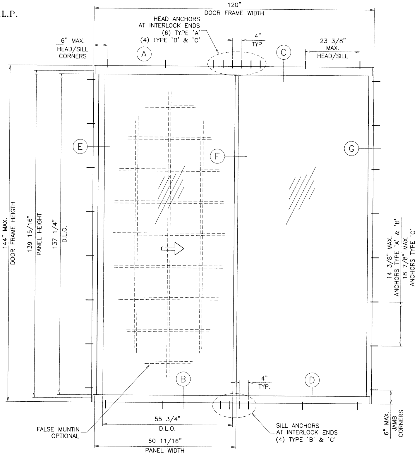
TYPICAL ELEVATION
