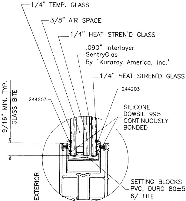
GLASS TYPE 'Bi' 1-3/16" OVERALL INSUL. LAM. GLASS
