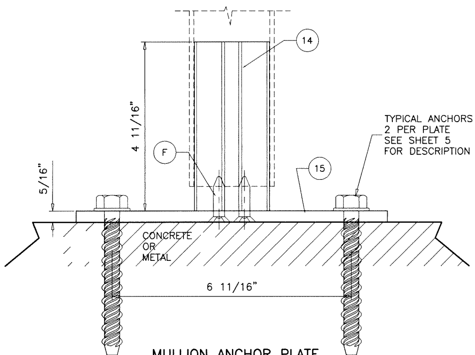
MULLION ANCHOR PLATE AT HEAD/SILL
