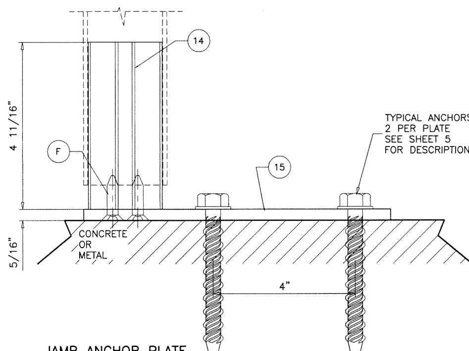
JAMB ANCHOR PLATE AT HEAD/SILL
