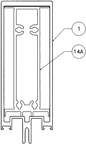
MULLION 'M2'
