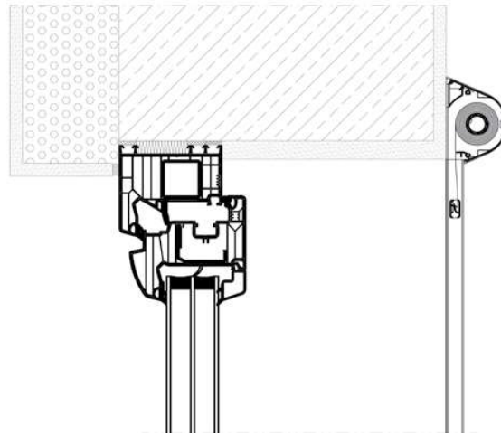
roller shutter – SRT SPACE
