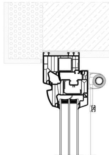
roller shutter – SRT FREE
