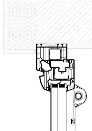
roller shutter – SRT FLAT
