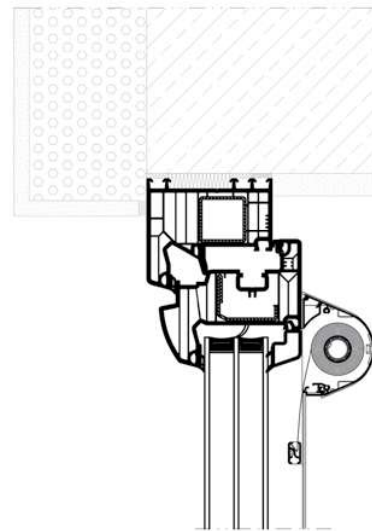
roller shutter – SRT FLAT MAXI
